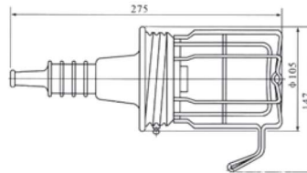
CSD3 - Lampu Jalan tanpa Kaca / Portable Light without Glass
