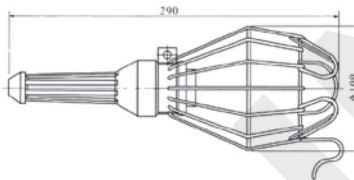
CSD3 - Lampu Jalan tanpa Kaca / Portable Light without Glass
